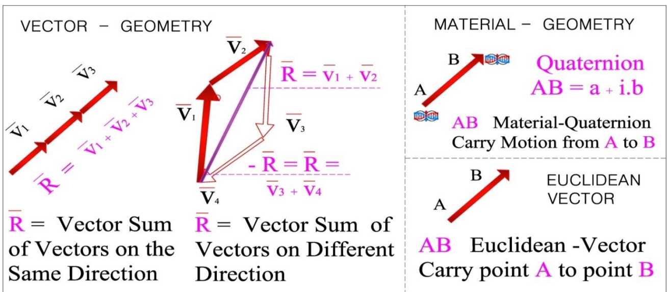
Figure-26.. In Euclidean-geometry , Point is nothing possessing Zero-magnitude and Infinite-directions. Two Points consist the Straight-line-segment , possessing |AB| - magnitude and the |A \rightarrow B| Directions .
