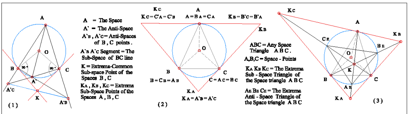
Figure.5. In (1) Concurrency points in and out of any circumcircle of triangle ABC . In (2) The Extrema Concurrency points of vertices of any triangle ABC . In (3) The Extrema Sub-Space and Anti-Space of any Space Plane-triangle ABC.
