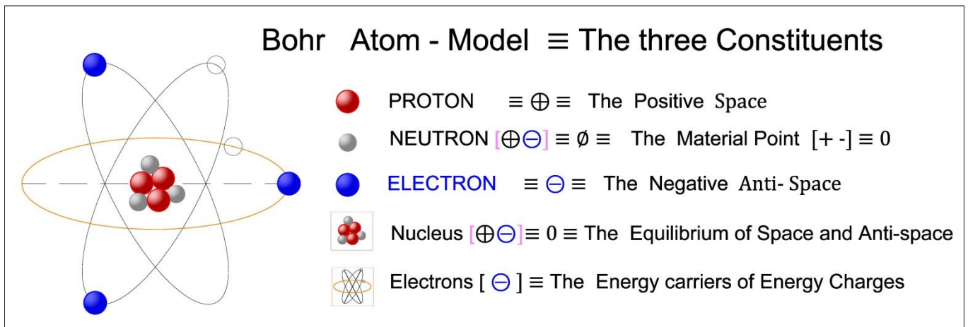
Fig-25. Proton , in Bohr-model , consists the \rightarrow Positive Breakage (+) of the three constituents , Electron consists the \rightarrow Negative Breakage (-) of the three constituents , Neutron consists the \rightarrow Equilibrium Material Point (+ -) of the Spaces and Anti-spaces . Nucleus consists the \rightarrow Equilibrium Positive Breakage Store , in Atom -Model Electron Orbits are the \rightarrow Equilibrium Negative Breakage Stores in Atom -Model Orbital Electron is the \rightarrow Moving-Charge-carrier of Energy in Atom -Model
