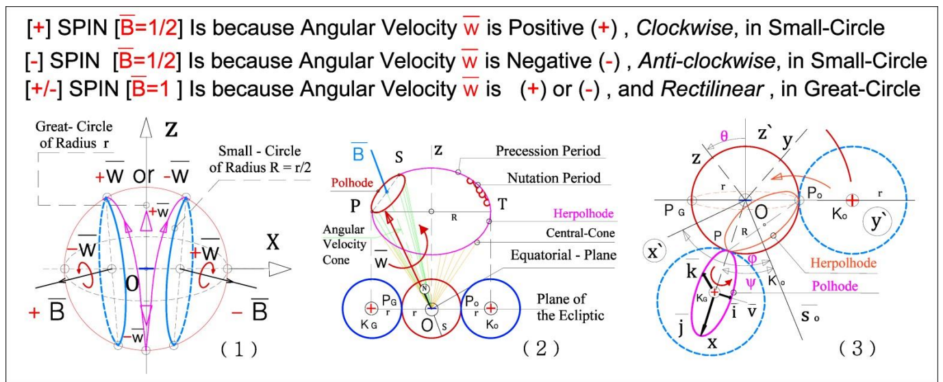
Figure .2.. In (1) The Glue-Bond pair of opposites [⊖ ⊕] of the Rectilinear motion in Great circles , creates rotation on circle of radius , r , with velocity v = w.r = \frac{2\pi}{T}.r = 2\pi r . f = [\frac{\sigma}{2}].(1+\sqrt{5}) , where frequency f = \frac{(1+\sqrt{5}) \cdot \sigma}{4\pi r} , Period T = \frac{4\pi r}{\sigma(1+\sqrt{5})} and \pm \sigma , are the two equal and opposite Centripetal , F_p , Centrifugal , F_f forces . Energy is \rightarrow E = h.f = \frac{(1+\sqrt{5}) \cdot \sigma h}{4\pi r} in Zero Wave-note .
