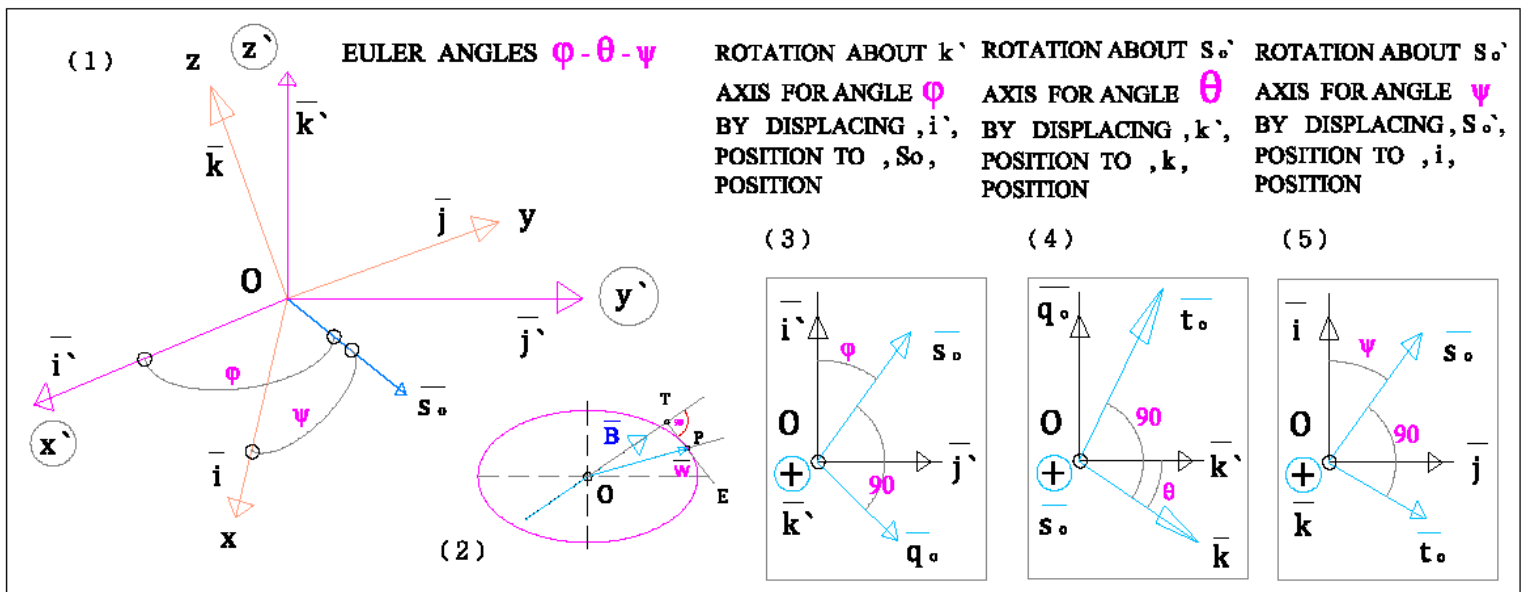
Figure.17. . In (1) are shown Euler angles { \phi, \theta, \psi } in a Fix-Three-Coordinate-System x, y, z through ,O, and one Movable x', y', z' at , O .
