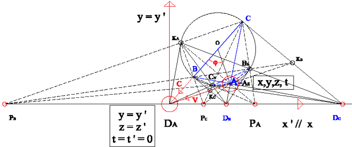
Figure.9. ABC is any Right-angled triangle at A (The Space), K_A K_B K_C triangle is the (Sub-Space), A_E B_E C_E triangle is the (Anti-space) respectively. The Instantaneous Pole P of rotation is off the Circle of diameter BC. The Poles of rotation lie on \{D_A - P_A\} Reference system.
