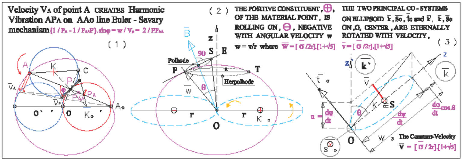
Figure.19. In (1) Material point AP , { the two circles \ominus \equiv K_0, K_0P - \oplus \equiv K, KP } of the Space point A (+) and Anti-point P(-) is rotating through point A_0 , which is the center of Common circle and form material angle \vartheta = \vartheta_A \cdot t = (\frac{V_A}{\sqrt{c^2 - v^2}}) \cdot t , CREATE the Cardioid Envelope curves generated by the above Vibrating -Velocity-Energy-Geometry-Segment , APA , on , AA_0 , rotating line.
