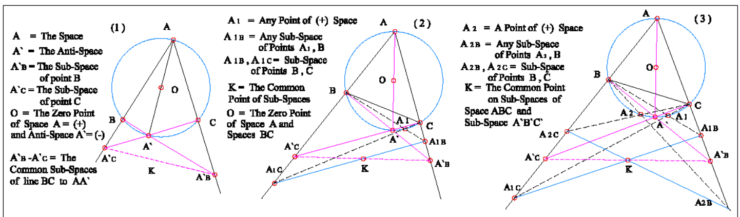
Figure.4.. The Coexistence of Space ABC and Anti-space A' , B' , C' in a Plane . The Spaces , Anti-Spaces of One Point is A \leftrightarrow A' , of Two Points B, C \leftrightarrow A'_B, A'_C , of Three Points ABC , the Plane , is ABC \leftrightarrow A' , A'_B , A'_C , and are the Extrema points on any circumcircle in triangle ABC . Discrete , on Geometry happens in all levels and Primary in STPL as shown below.
