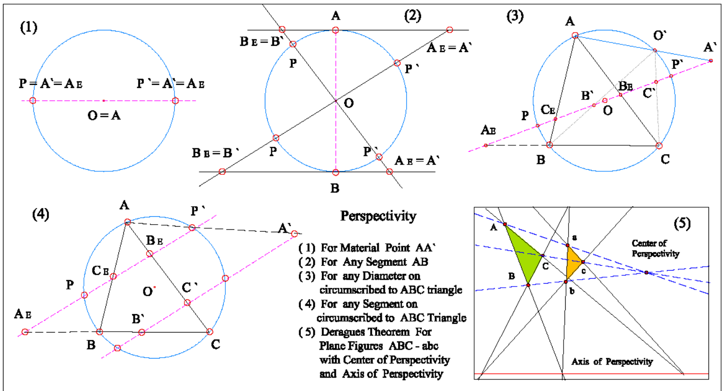
Figure.3.. Pole and Axis of Perspectivity for Points, Sectors, Planes, Volumes. The two Perspective Desargues triangles ABC - abc with their Axis and Center of Perspectivity.
