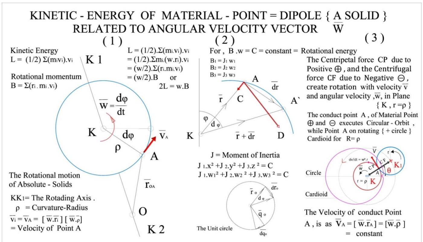
Figure.13.. The Cycloidal motion in , Material Point \equiv The monad is Dipole \equiv [\oplus \ominus] = \emptyset = K_R AK_{R=r} where \rightarrow K_R \equiv [\oplus] \leftrightarrow K_R \equiv [\ominus] \rightarrow \equiv 0 . The total torque becomes from \pm Spin which equilibrium in System of circle K_R , Evolute circle K_R , as Cardioid of the same center. In (3) the Flexible - String OA is stretched under equilibrium Tension = \pm\sigma and rotated around O center with a constant angular velocity , w , and is vibrated in Normal modes .
