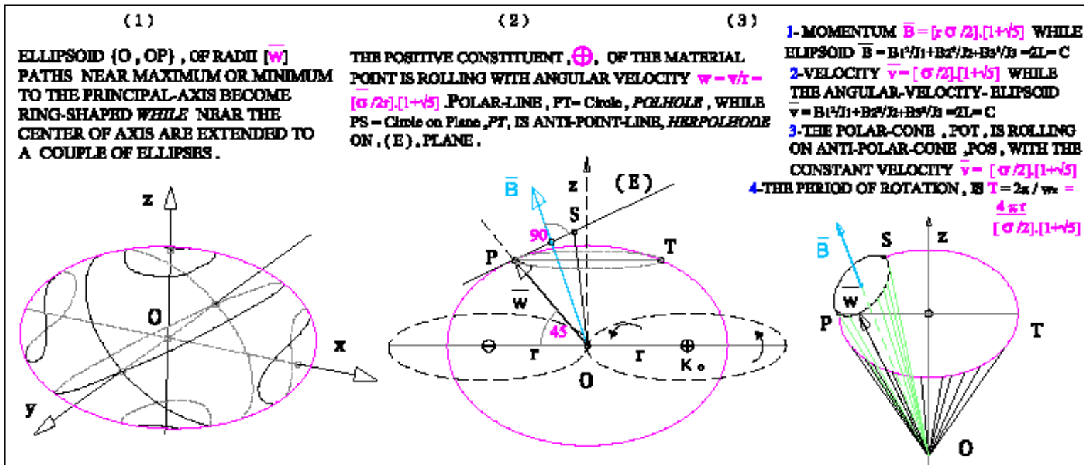
Figure.18.. In (1) , are shown Paths near maximum or minimum to Principal axis from where become-ring shaped or Small-circles , while near the center of axis extend to a couple of ellipses or Great circles . Rotating on small circles is created the \pm \frac{1}{2} \text{ Spin} \equiv \bar{B} In (2) is shown Rotation with angular-velocity \bar{w} , 45^\circ to the instantaneous material axis OP \equiv [\oplus \leftrightarrow \ominus] of rotation where point P is the , Nib , of Angular-velocity vector \bar{w} and Sweeps-Out at OP slant height of the Central , POT-Cone , with \bar{w} = \frac{v}{R} . In (3) are shown Polhode , circle PT , Herpolhode , PS circle in plane E . Polhode-Cone POT is rolling on the Fixed- Herpolhode-Cone POS , with the constant velocity |\bar{v}| = \frac{\sigma}{r} [1 + \sqrt{5}] dependent on Pressure , \sigma , of the two material constituents .
