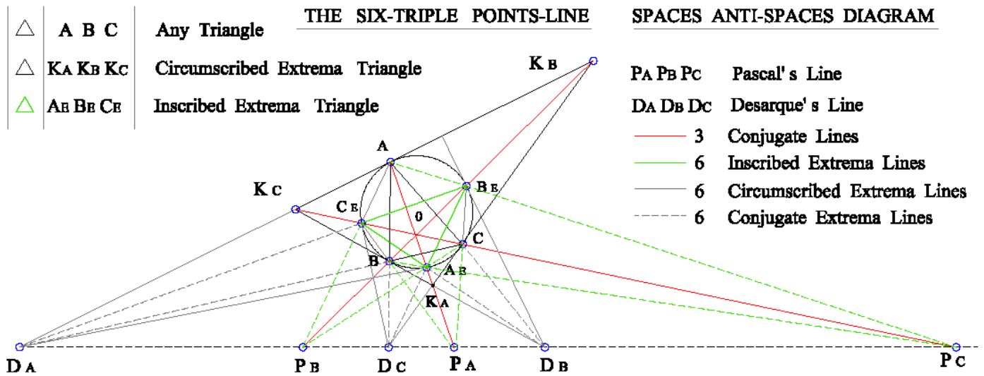
Figure.6.. The Six, Triple Concurrence Points, Line . [STPL] → D A , D B , D C - P A , P B , P C [ ABC ≡ The Space ] , [ A E , B E , C E ≡ The Anti-Space ] , [ K A , K B , K C ≡ The Sub-Space ]
