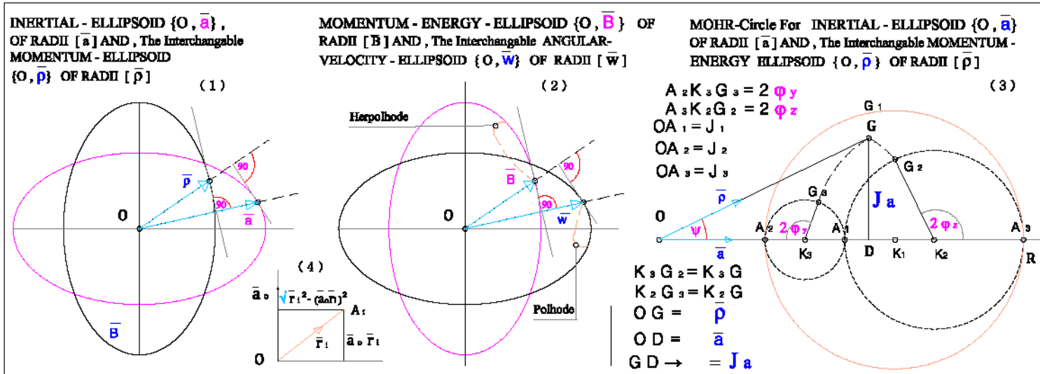
Figure.16.. In (4) is shown the Geometrical-meaning of \bar{a}_0 \bar{r}_1 and \sqrt{r_1^2 - (\bar{a}_0 \bar{r}_1)^2} terms.
