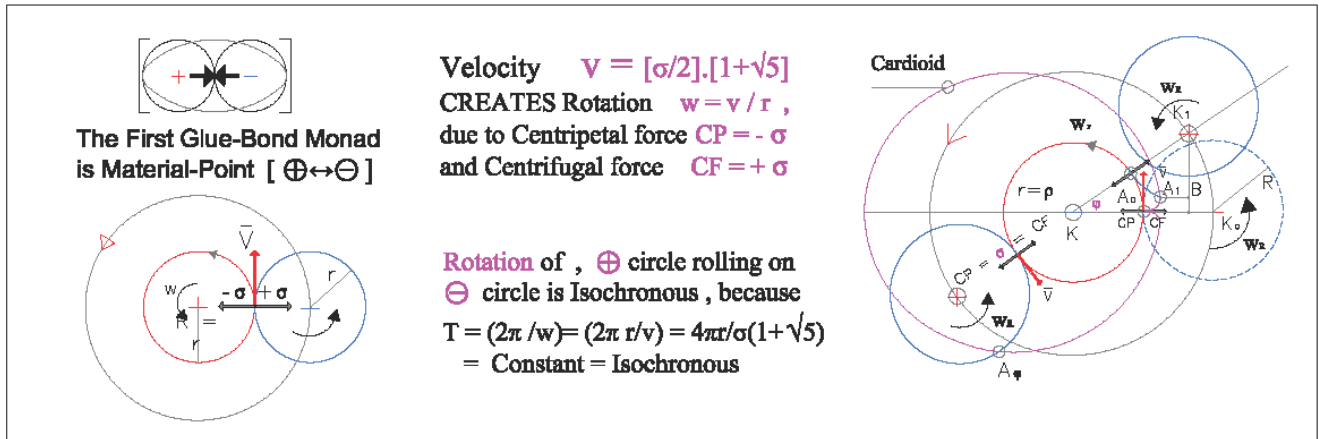
Figure.12.. The Isochronous Rolling of circles[⊕⊖] ( in Material Point, due to Glue-Bond {+σ-σ} ), happens because the period T = \frac{4\pi r}{\sigma(1+\sqrt{5})} = \text{Constant} , therefore and Isochronous.
