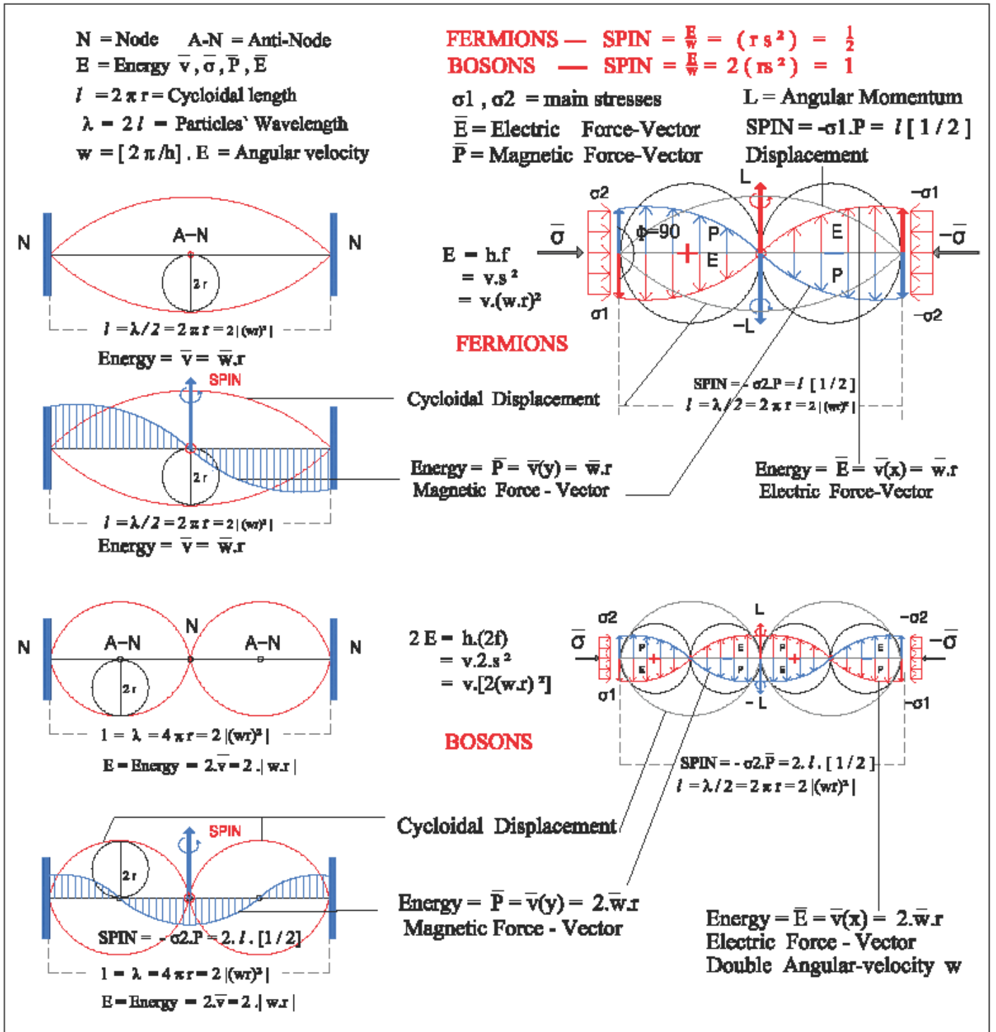
Figure.21. The Energy \bar{B} = \frac{h}{2\pi} = \text{Spin} = \frac{h.f_1}{w} as velocity, v = (wr) in cave, l , is the Spin \frac{1}{2} , while Doubled \bar{B} = \frac{h}{2\pi} = \text{Spin} = 2 = \frac{h.f}{w} = 2.\bar{B} , in the same cave, l , then \rightarrow f = 2.f_1 i.e. In the same cave, l , Energy is quantized as \frac{1}{2} / 2.\frac{1}{2} = 1/3.\frac{1}{2} = 1.5/4.\frac{1}{2} = 2, \dots n \frac{1}{2} and so on, depending on the number, n , of Wave-notes in cave, l .
