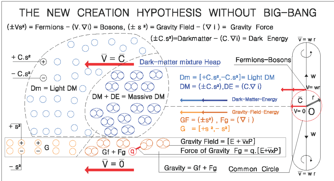
Fig-24. The Cause Expansion of the Universe , is the continuous and simultaneous Rolling of mixture Heap [ DE-DM ] , The Fragments Heap , on the Rest Gravity-field [G f + F g ] as the Base of rolling.
