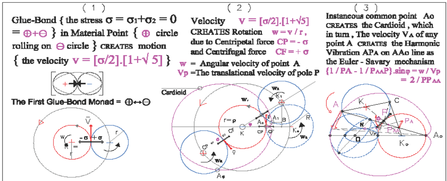
Figure.14.. Pole of rotation P , on STPL line AP A , is the Instantaneous centre of rotation for [⊕] , Space on [⊖] Anti-space , through Sub-space, ∅, and or , every couple of lines between Spaces and Anti-spaces . Cardioid is the envelope of circles ( K 0 ,R ), ( K , r = R ) whose centres K 0 , K lie on a given circle ( P , PA 0 ) which pass through a fixed point , A 0 , on the given circle ( P , PA 0 ) .Nutation happens at ,N, common point. Analytically in [58] .
