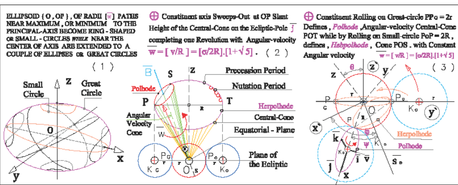
Figure.20. In (1) , are shown different Paths near maximum or minimum Principal axis from where become-ring shaped or Small-circles while near the center of axis extend to a couple of ellipses or Great-circles .For a constant Angular-velocity , w , and by changing torsional momentum , B , only then Infinite curves are possible for the motion .
