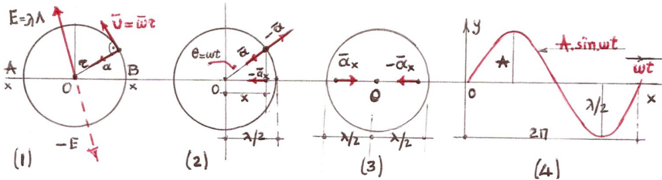
Figure.23. In (1) , are shown Velocity , |\vec{v}| = w.2r = \frac{2\pi}{T}.r = 4\pi r. f = [\frac{\sigma}{2}].(1+\sqrt{5}) , Angular velocity |\vec{w}| = \frac{\sigma}{2r} [ 1 + \sqrt{5} ] and Frequency , f = \frac{(1+\sqrt{5}).\sigma}{4\pi r} in cave , r .
