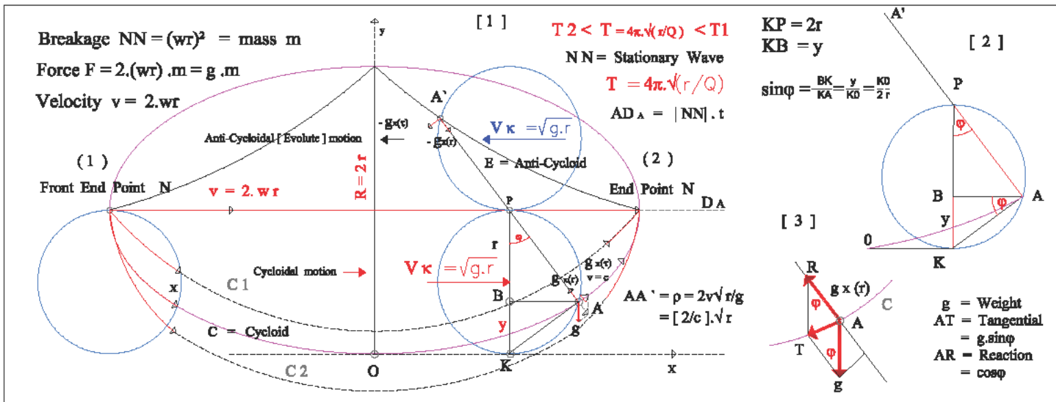
Figure.11. The Cycloidal motion in, Material Point ≡ The monad is Dipole ≡ [⊕⊖] = ∅ = AA' where \rightarrow A \equiv [\oplus] \rightarrow A' \equiv [\ominus] \rightarrow |AA'| \equiv \emptyset \equiv The Brachistochrone Curve C ≡ N1 → N2. Motion on Curve C1 acquires a period T_1 > 4\pi\sqrt{r/g} , while on C2 T_2 < 4\pi\sqrt{r/g} which is not Isochronous.
