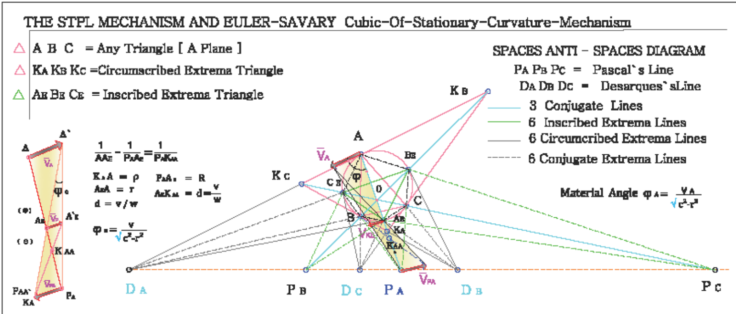
Figure.7.. ABC is any triangle ( The Space ) , K_A K_B K_C triangle is the ( The Sub-Space ) , A_E B_E C_E triangle is (The Anti-space) respectively . The Instantaneous Pole P \equiv A_E of rotation is off the circle on AA_E axis .Inscribed to ABC circle is Common circle of STPL- \{D_A-P_A\} mechanism The Reference System \{D_A- P_A\} \equiv [R] (x',y',z', t') moves with velocity , \bar{v} , parallel to , x-x' , axis with respect to the fixed and Absolute System \{D_A- O\} \equiv [S](x,y,z, t) . The Space point , A , moving on (p) curve , and Anti-Space point A_E moving on (ε) curve are rolling on the same Sub-space circle (O,OA) \equiv (O,OA E ) which is the common cave-circles of Material Geometry in STPL - \{D_A-P_A\} mechanism .
