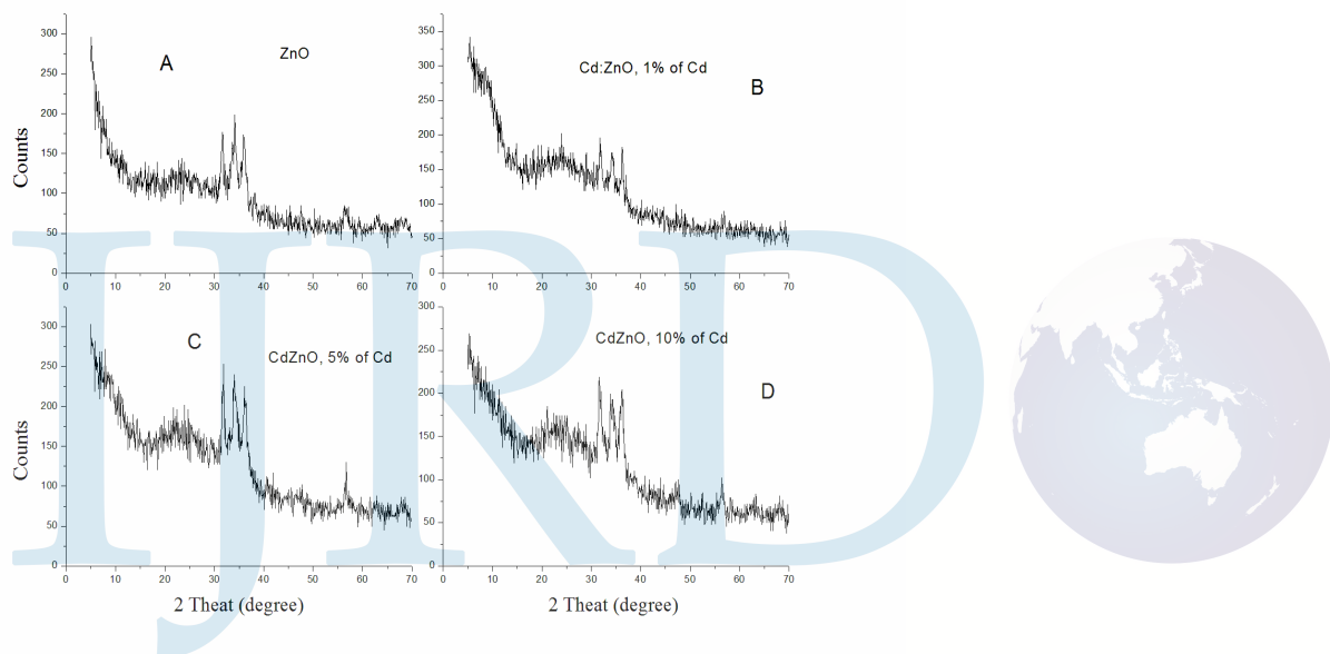
Figure 1: XRD of ZnO: Cd thin films before and after Cd doping.
