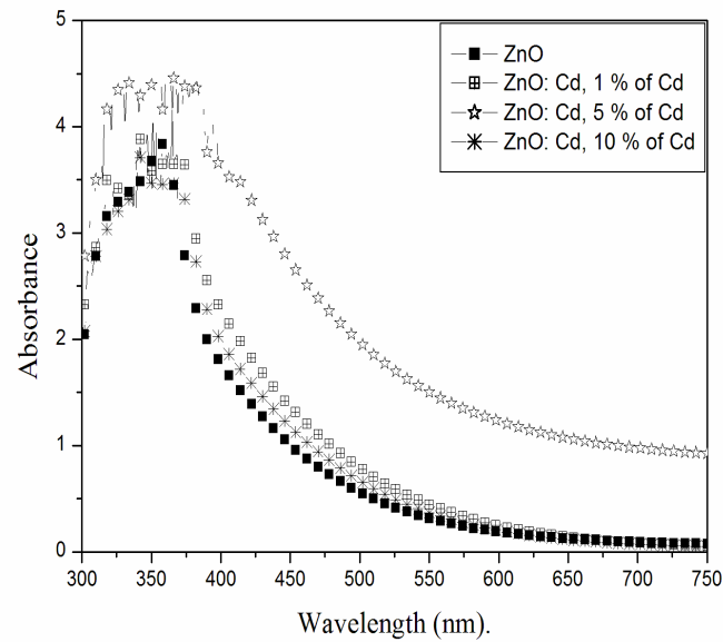
Figure 2: optical absorption of ZnO: Cd.
