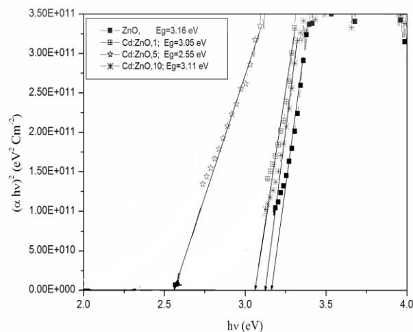
Figure 3. Optical band gap of ZnO: Cd thin films.
